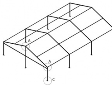
Sidewall downside bar 墙底压布杆
